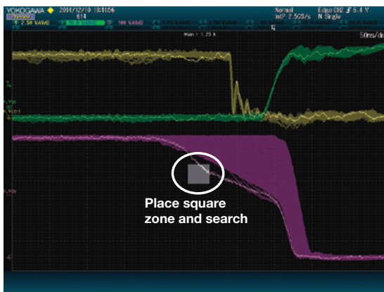
Searching for waveforms that pass through or do not pass through a rectangular zone placed on screen.
